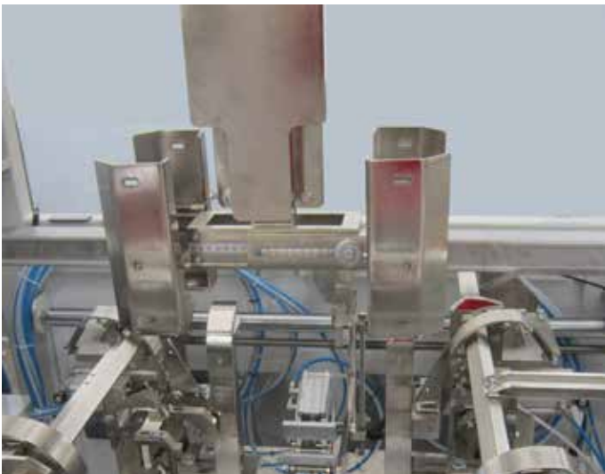
ADJUSTABLE PRESS / PRESSA MULTIFORMATO
